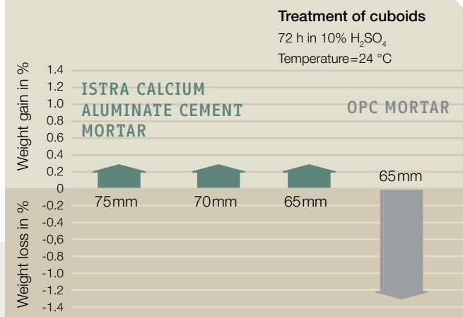
Figure 5: Weight loss Istra 40 and OPC mortar
